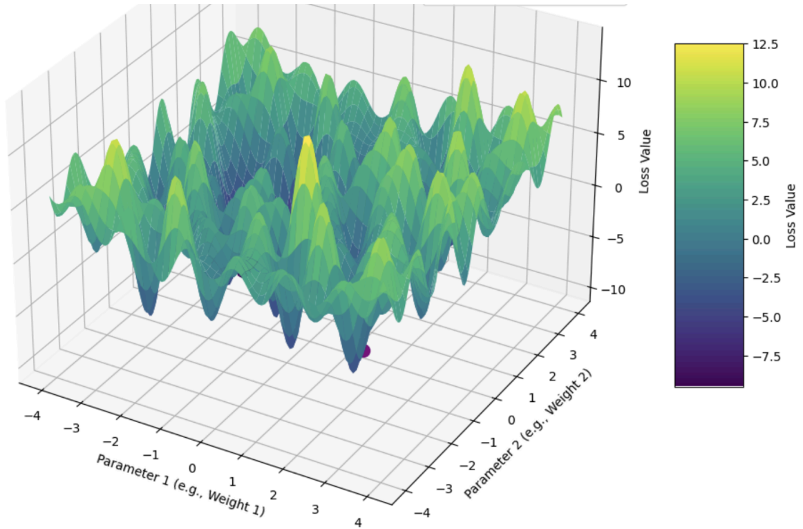
Figure 1: Example of a loss surface of a 2-neuron neural network. Higher points on the surface represent higher error of the neural network prediction based on which weights (shown as x and y axes) the network chose. The optimizer will update weights to move towards the bottom of the loss surface - this represents neural network learning to minimize the prediction error. An optimizer that has a better way of traversing the loss surface (searching for lower loss) will train the neural network faster.
