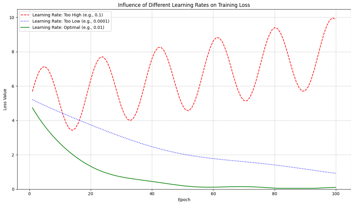
Figure 2: Example of 3 learning rates. A too high learning rate (red) results in the loss (error) increasing, and the neural network is unable to improve due to updates to weights
